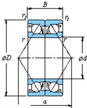
■ Mounting dimensions
